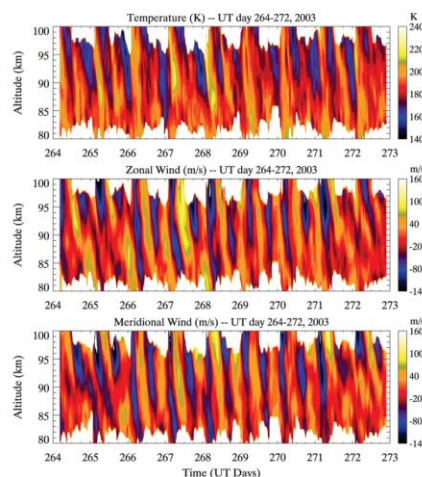
Laser beams into the night sky for the MLT science TUV contours; CSU Lidar
