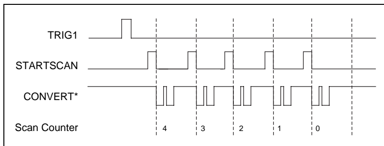
Figure 4-17. Typical Posttriggered Acquisition
