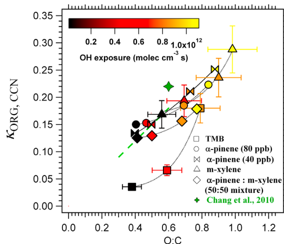
Figure 2. \kappa_{ORG,CCN} vs O:C for the laboratory SOA particles generated in this study. The \kappa_{ORG,CCN} for ambient OOA and the parameterization \kappa_{ORG,CCN} = (0.29 \pm 0.05) \cdot O:C of Chang et al. [2010] (dashed line) are also plotted. Error bars (shown for m-xylene and TMB SOA only) represent measurement precision of \pm 15\% in \kappa_{ORG,CCN} and \pm 15\% in O:C.
