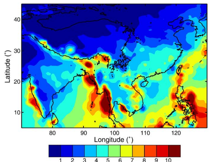
Fig. 2. Annual mean (1920–1980) precipitation rate (mm/day) over Southeast Asia from the Legates Surface and Ship Observation of Precipitation dataset (Legates and Willmott, 1990). Black contour lines denote elevations of 0 m and 2000 m. Note high precipitation rates along the Himalayan front and in southeast China resulting from South Asian and East Asian monsoon activity.
