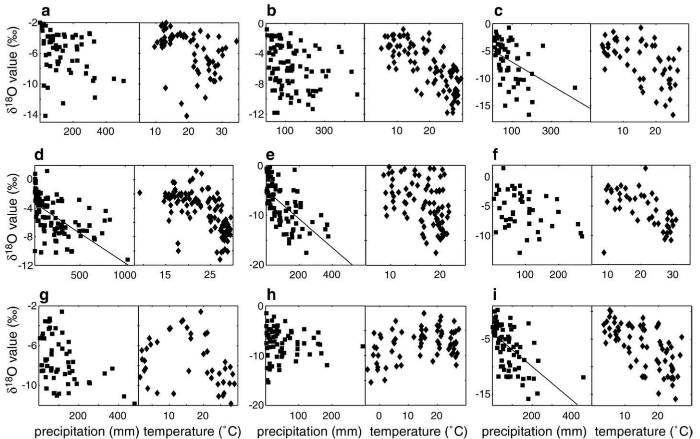
Fig. 4. Monthly total precipitation (mm, squares) and monthly mean temperature ( ^{\circ}\text{C} , diamonds) versus monthly mean \delta^{18}\text{O} values (‰) for stations at (a) Fuzhou, (b) Guilin, (c) Guiyang, (d) Hong Kong, (e) Kunming, (f) Liuzhou, (g) Nanjing, (h) Shijiazhuang, and (i) Zunyi, whose locations are shown in Fig. 1. Linear regressions used in the calculations in the Discussion are shown in black lines for stations at Guiyang, Hong Kong, Kunming, and Zunyi.
