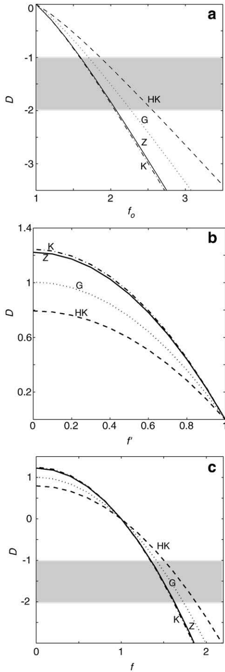
Fig. 5. Calculated annual average weighted \delta^{18}\text{O} values relative to modern, D , as a function of (a) f_0 for f = 1 , (b) f for f_0 = 1 , and (c) f = f_0 = f calculated using Eq. (6) relative to modern values. Dotted lines (marked 'G') are calculations for station at Guiyang, dashed lines (marked 'HK') are for Hong Kong, dot-dashed lines (marked 'K') are for Kunming, and solid lines (marked 'Z') are for Zunyi. Gray bands in (a) and (c) indicate minimum \delta^{18}\text{O} values in the records from Dongge and Hulu caves (2004). Values for a and P_0 in Eq. (2) for the stations shown are: a = -0.025 , P_0 = 80.4 (Guiyang); a = -0.0081 , P_0 = 196.1 (Hong Kong); a = -0.03 , P_0 = 83.0 (Kunming); and a = -0.030 , P_0 = 81.5 (Zunyi). Units of a and P_0 are \text{‰}/\text{mm}/\text{month} and \text{mm}/\text{month} , respectively.
