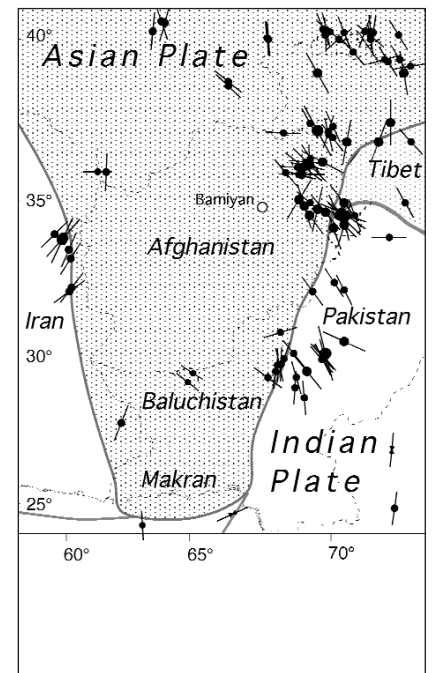
Figure 7.2b (Low) Principal stress directions from earthquakes reveal largely oblique compression on the eastern and western edges of Afghanistan, a 1200 km southward promontory of the Asian plate (stippled). Data from World Stress Map.
