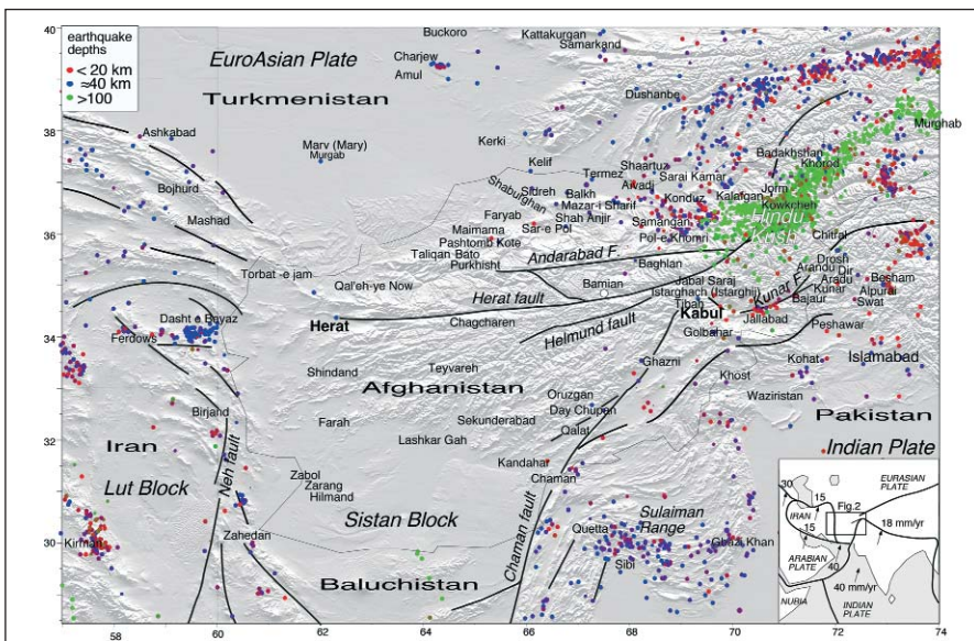
Figure 7.2a (Up) A map of Afghanistan showing prominent faults, and major earthquakes described in the article. In 1956 a significant earthquake occurred near Bamiyan in the block bounded by the Andarabad fault and the Herat fault.
