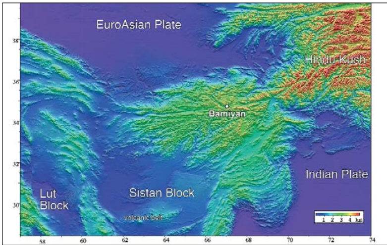
Figure 7.1a Bamiyan lies at the centre of the mountains of central Afghanistan on an ancient trade route linking east to west through the valley of the great Herat fault.
